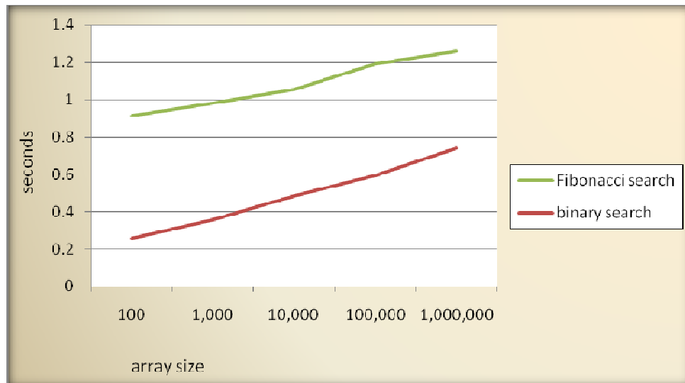
The results for 200 pseudorandom numbers, each sought for 10,000 times
